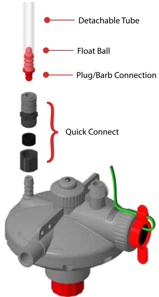
Threaded Quick Connect Part #7TEF024
